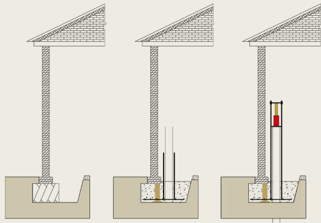
Boulder-foundation change
